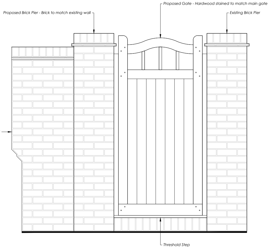
Proposed Gate - Detail B
