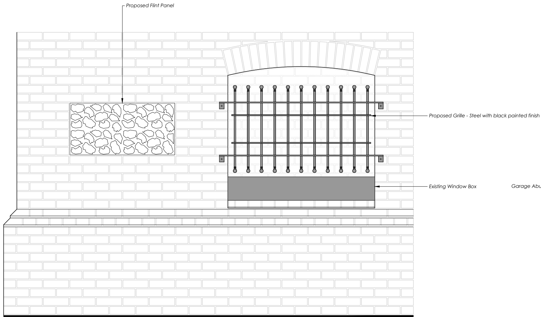
Proposed Grille & Flint Panel - Detail A
