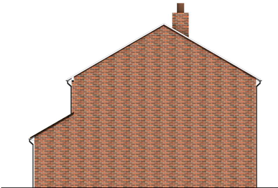
PRO. SIDE (SOUTH) ELEVATION 1:100
