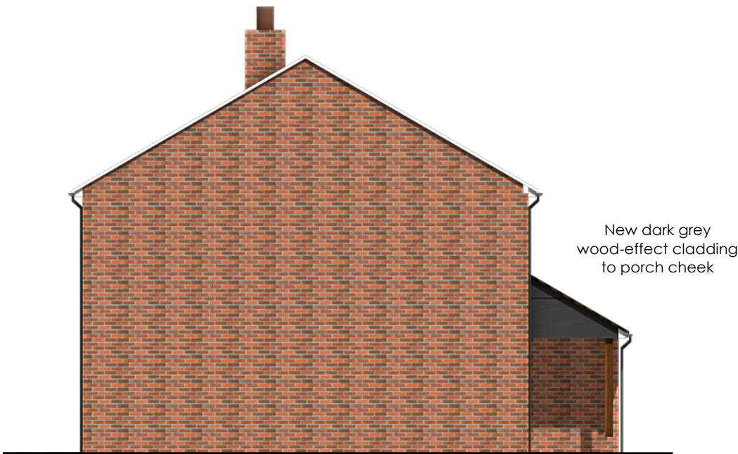
PRO. SIDE (NORTH) ELEVATION 1:100
