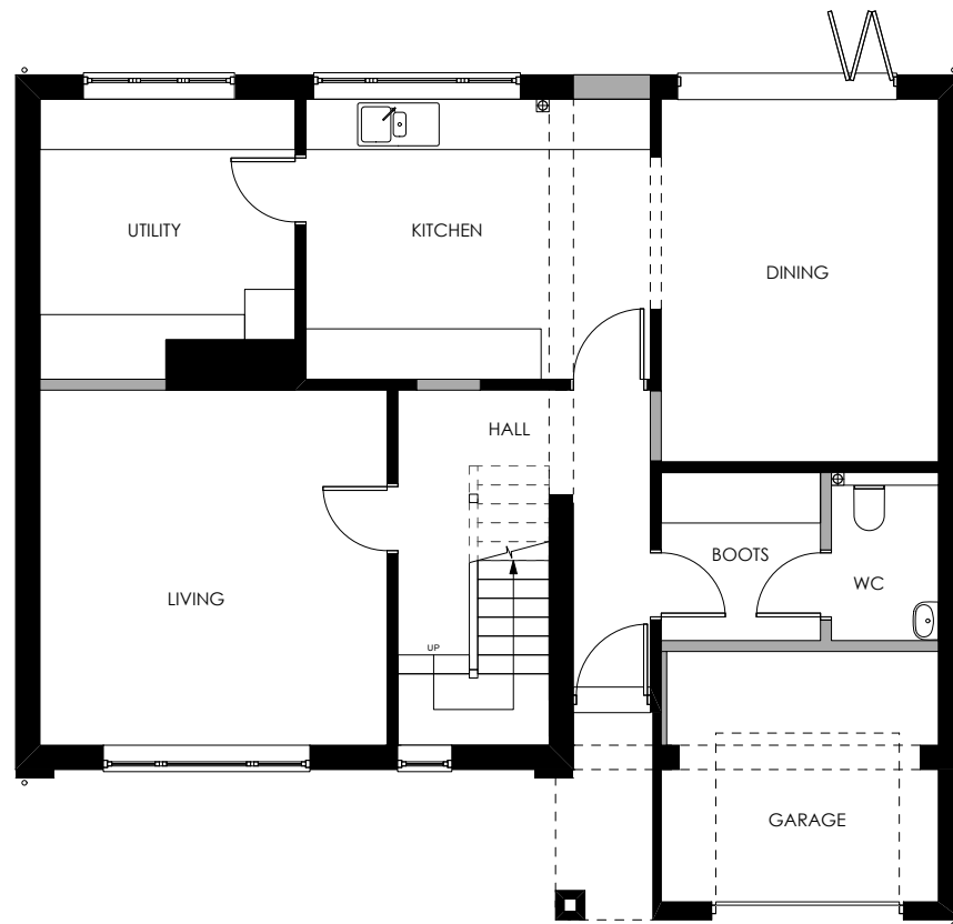
PRO. GROUND FLOOR PLAN 1:100
