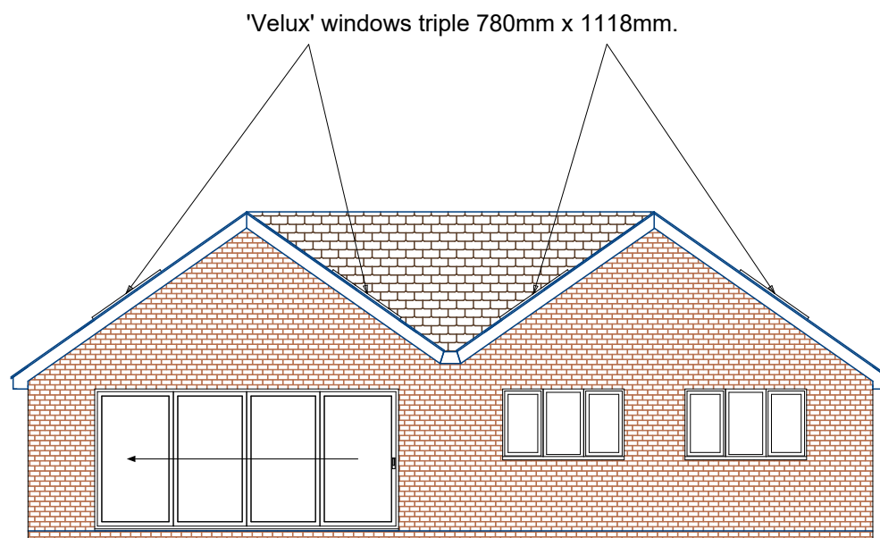
Proposed Rear Elevation (Revised)
