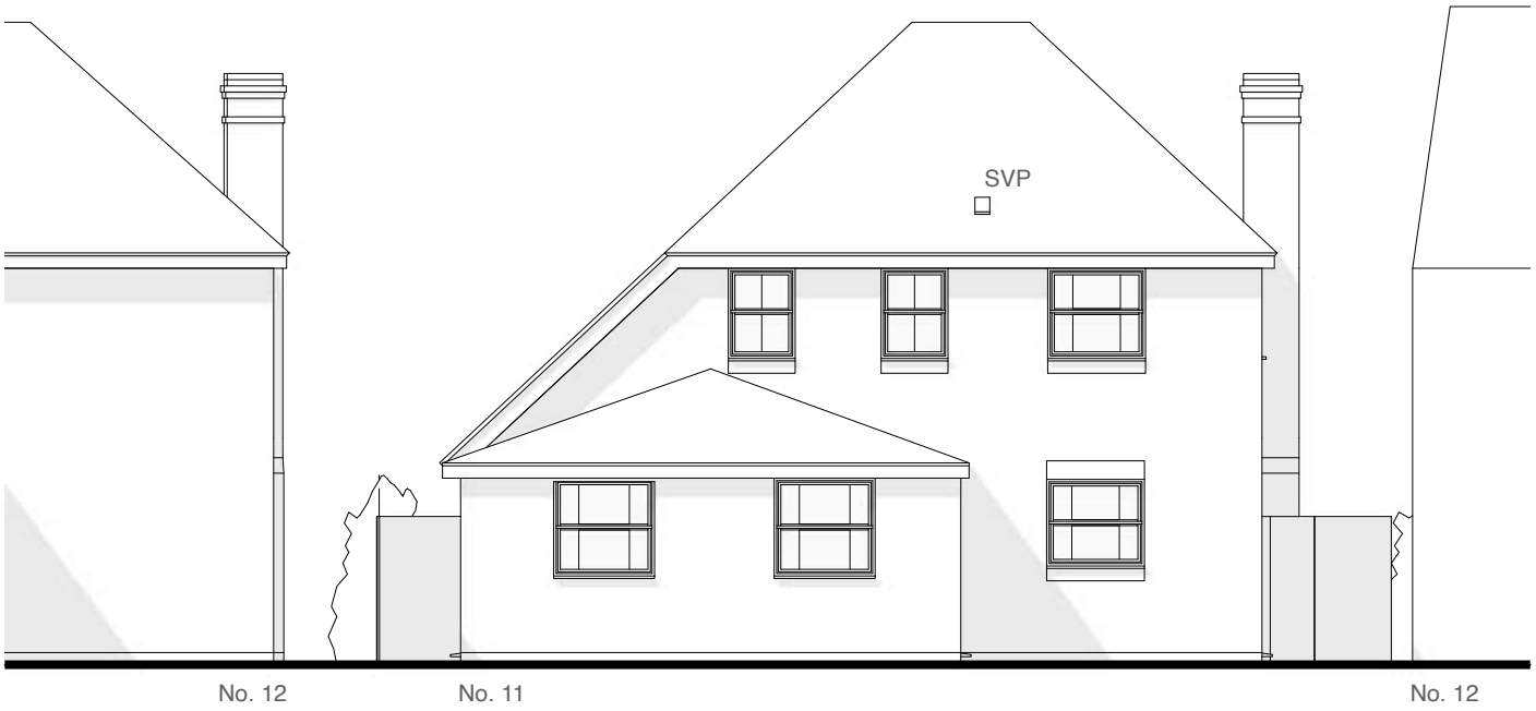
Rear elevation
