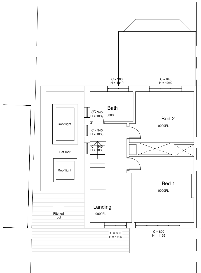
First Floor 1:100
