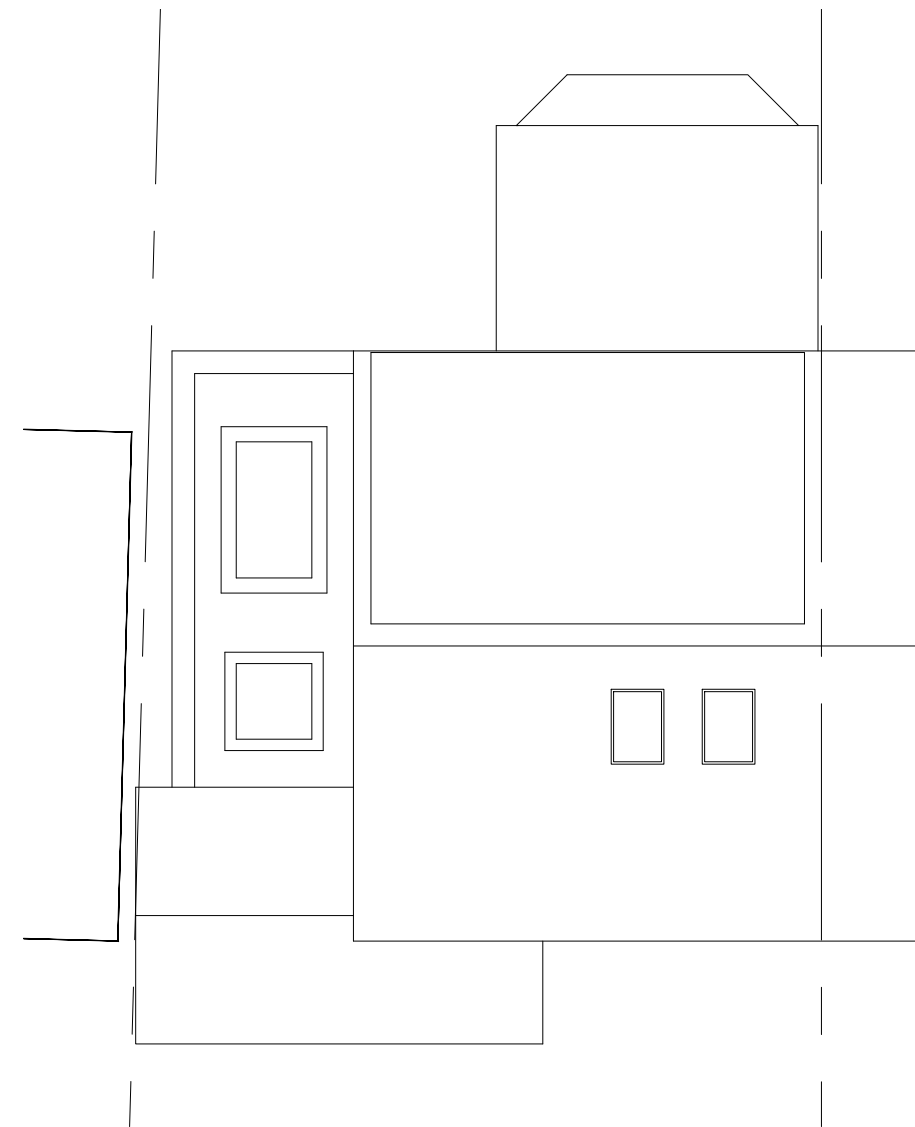
Roof Plan 1:100
