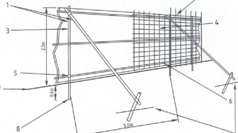
BS:5837 Figure 2 - Tree Protection Fencing structure around RPA
