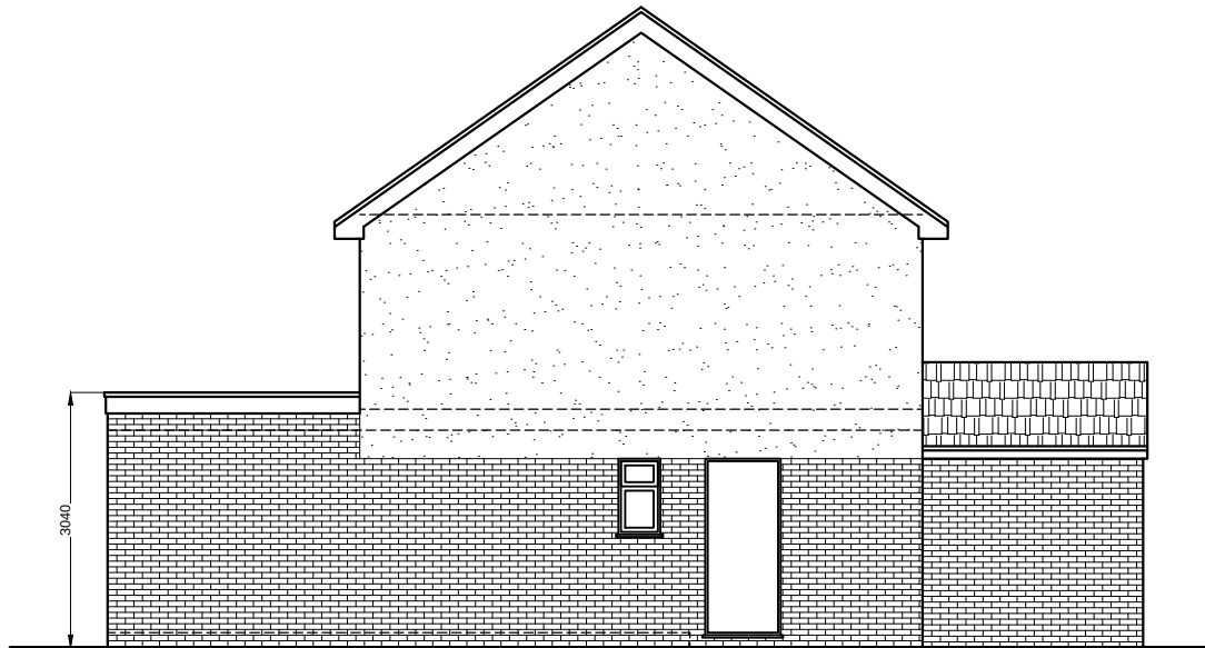
Proposed Left Side Elevation Scale: 1/100
