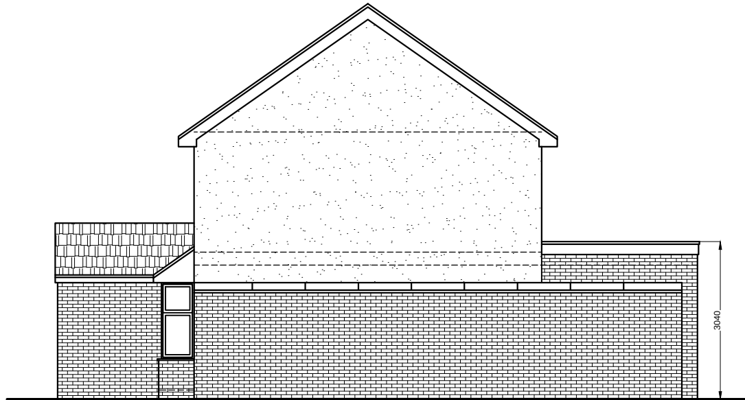
Proposed Right Side Elevation Scale: 1/100
