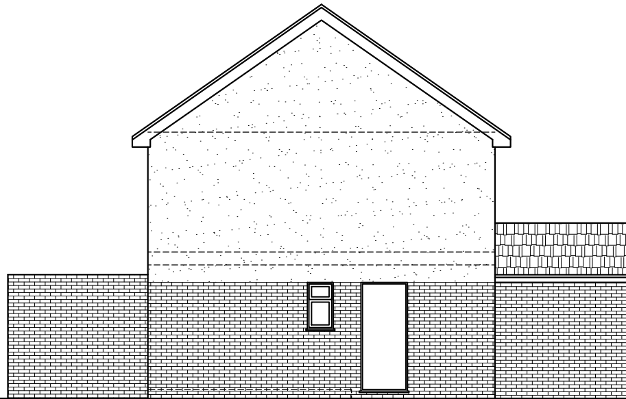
Existing Left Side Elevation Scale: 1/100
