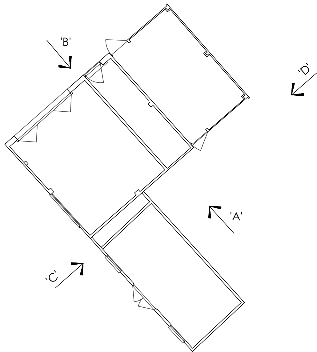
EXISTING ANNEXE BUILDING PLAN.
