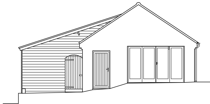
EXISTING ELEVATION 'B'.
