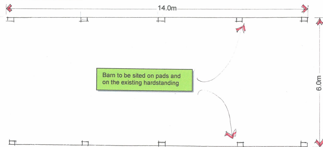
Floor plan
