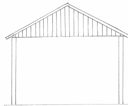
Southwest elevation
