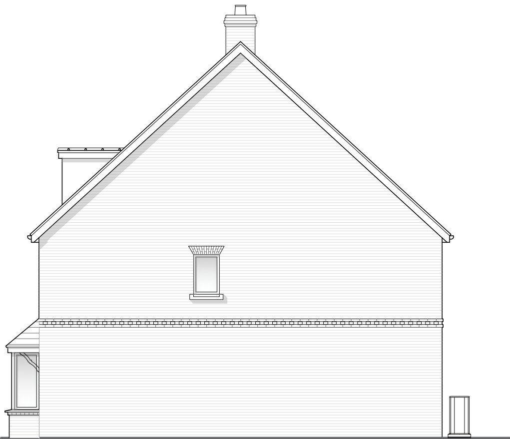
Elevation D
