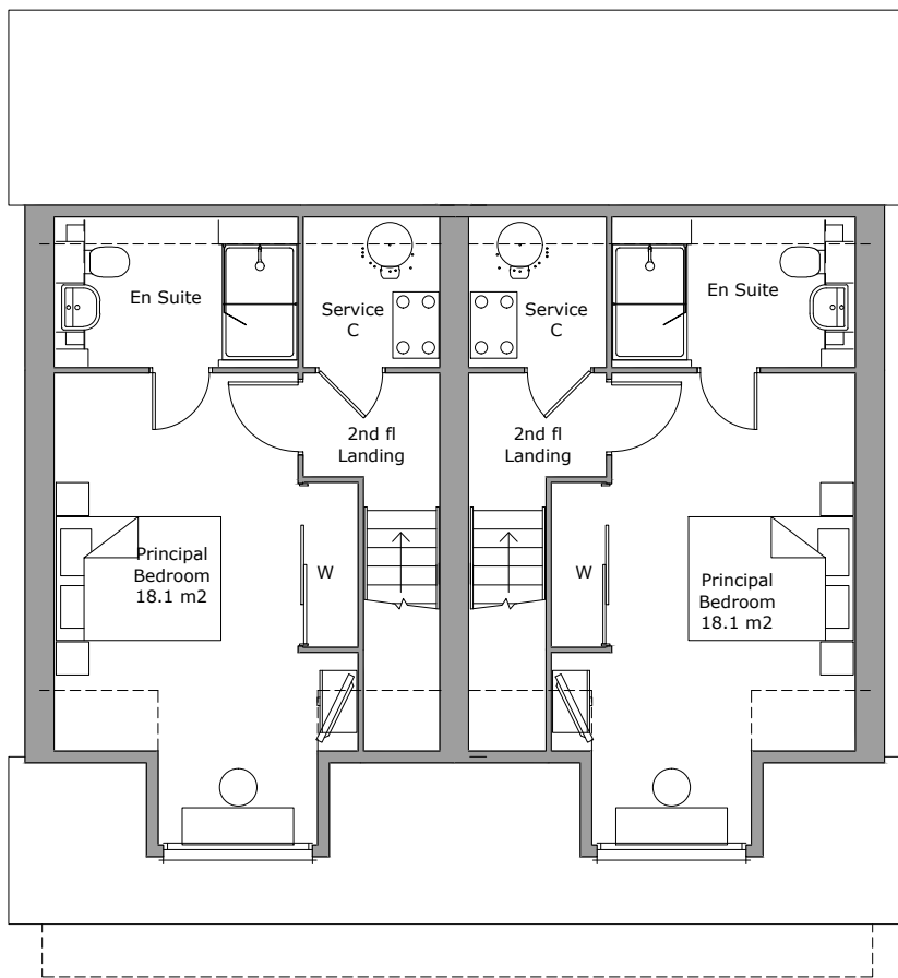
Second Floor Plan Area 32.6m²
