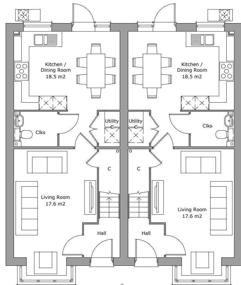
Ground Floor Plan Area 48.2m²
