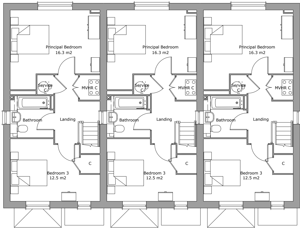
Second Floor Plan Area 46.8m²
