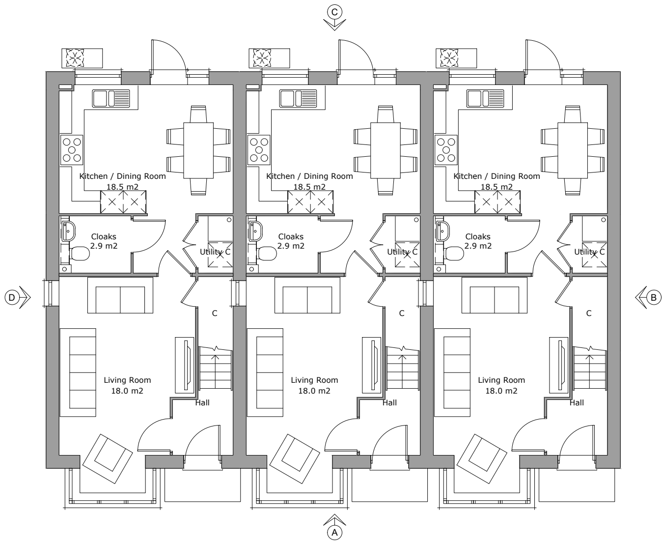
Ground Floor Plan Area 48.6m²
