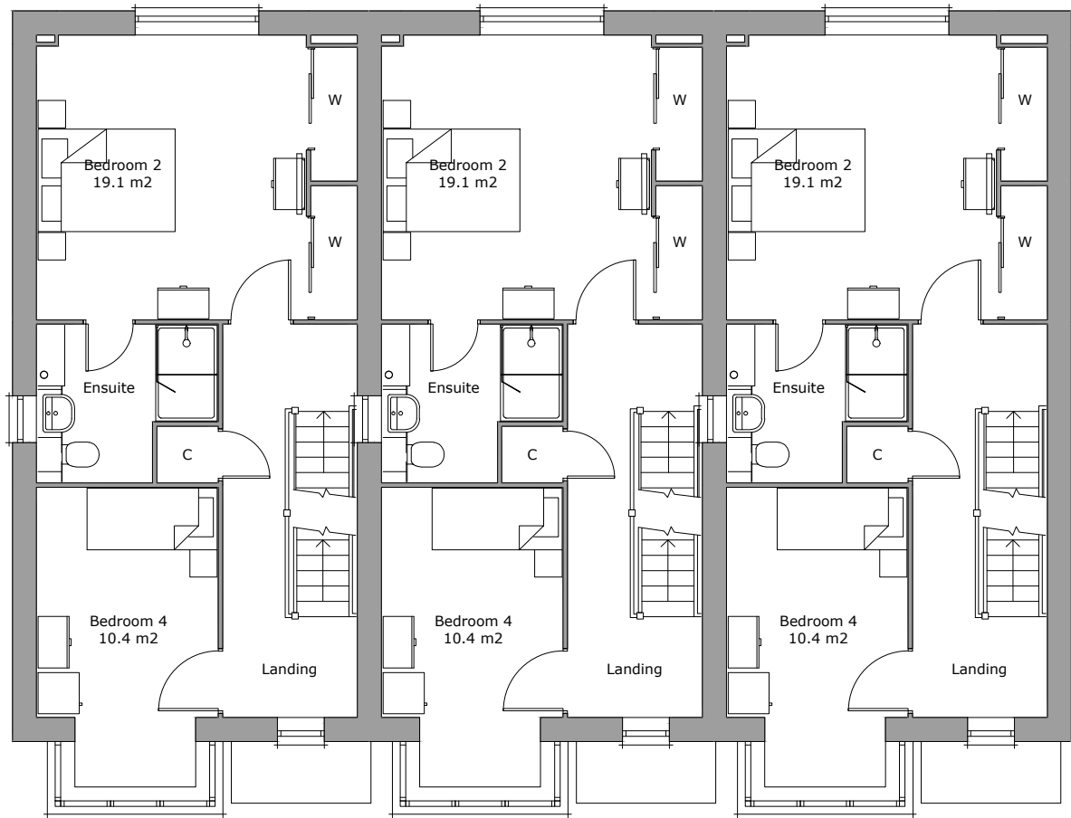
First Floor Plan Area 48.6m²
