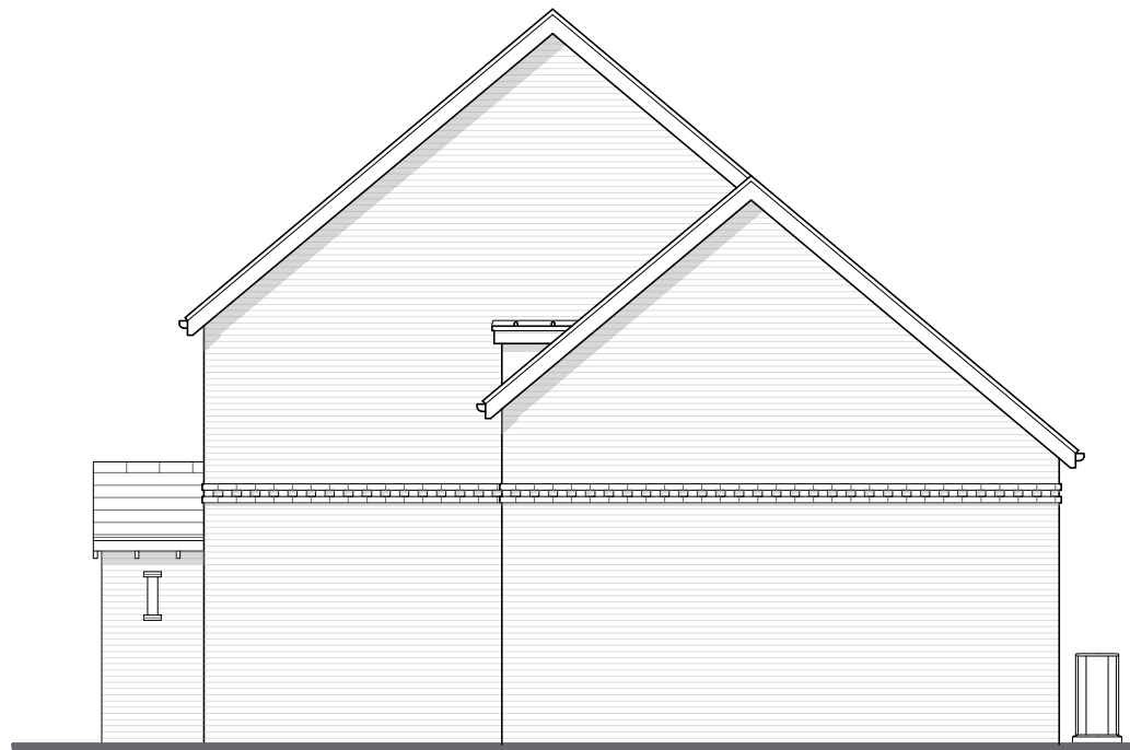
Elevation D
