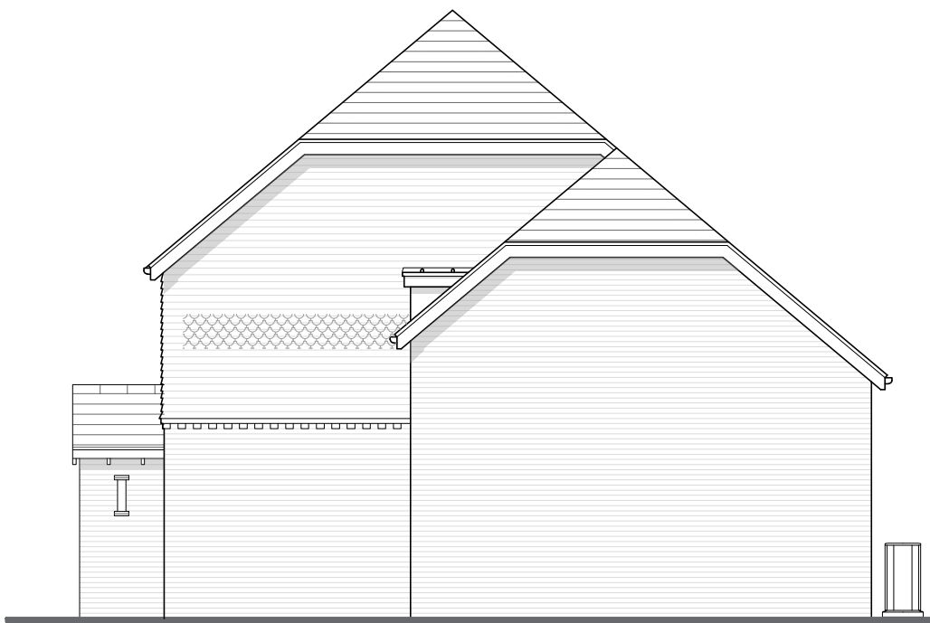
Elevation D
