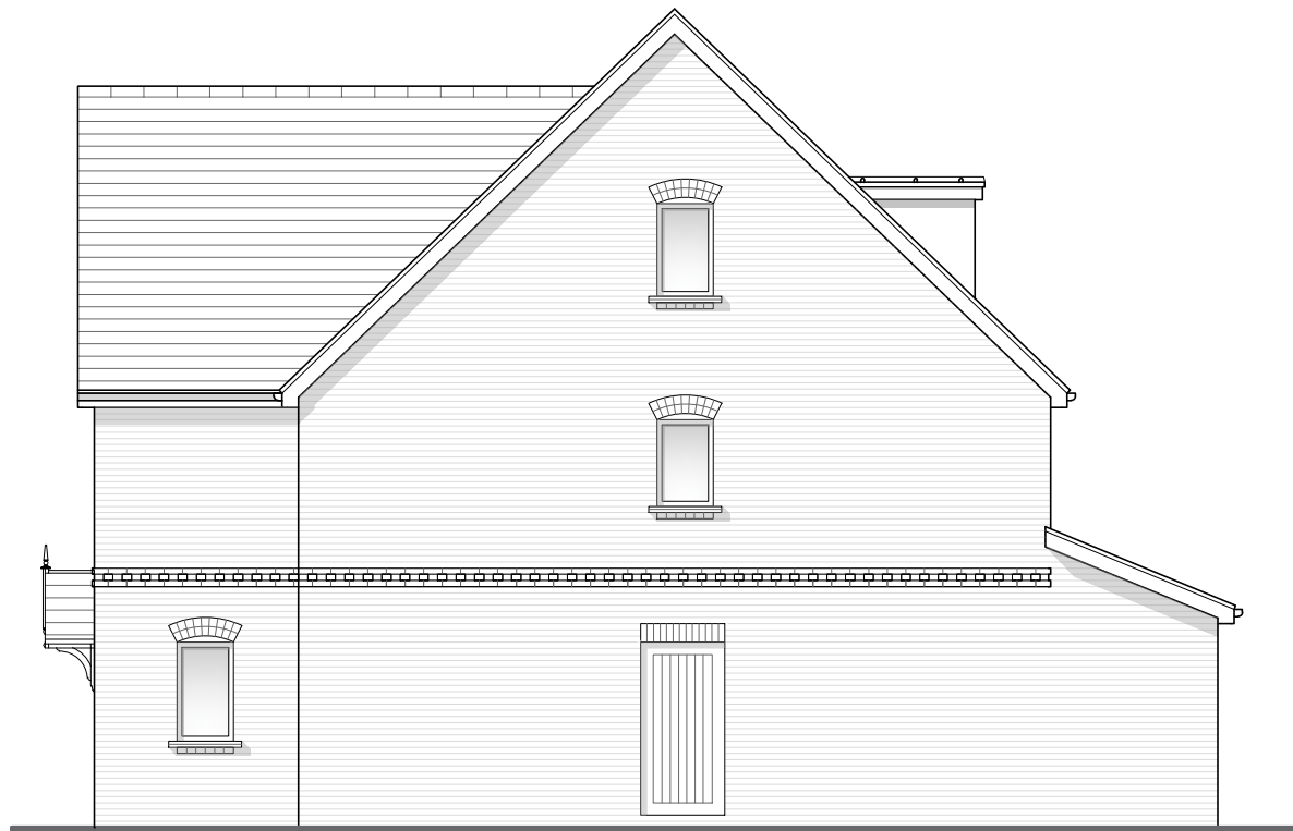
Elevation D
