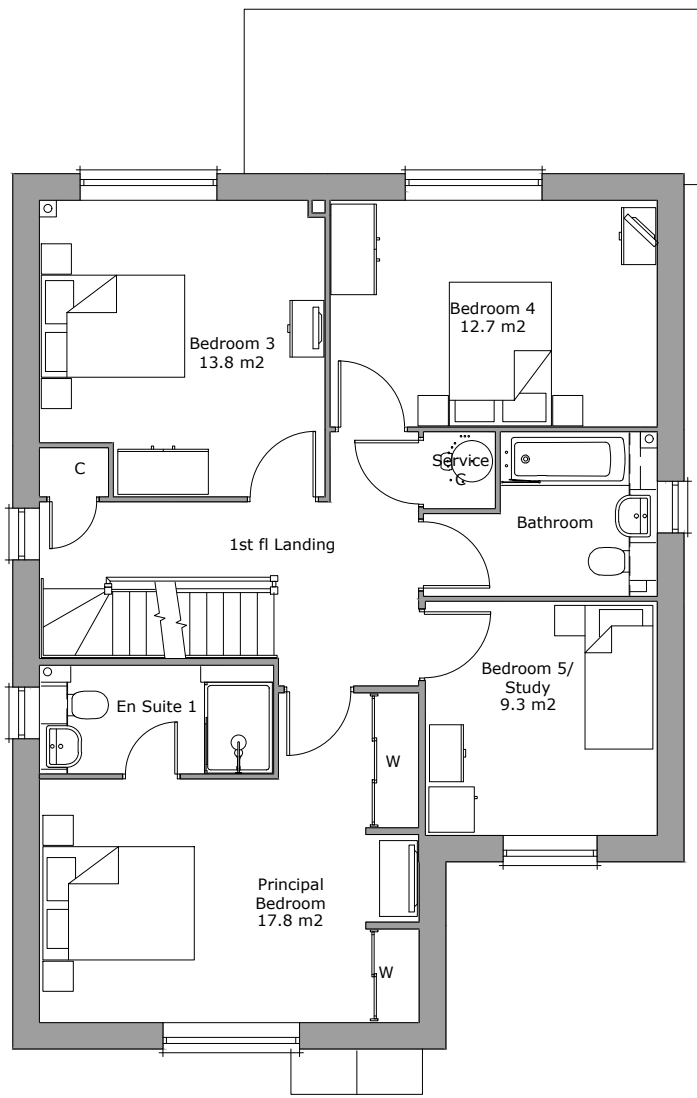
First Floor Plan Area 81.1m²
