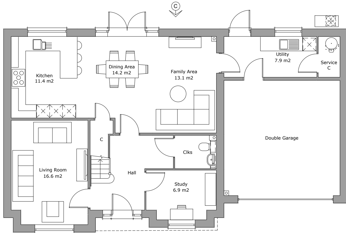
Ground Floor Plan Area 90.9m²
