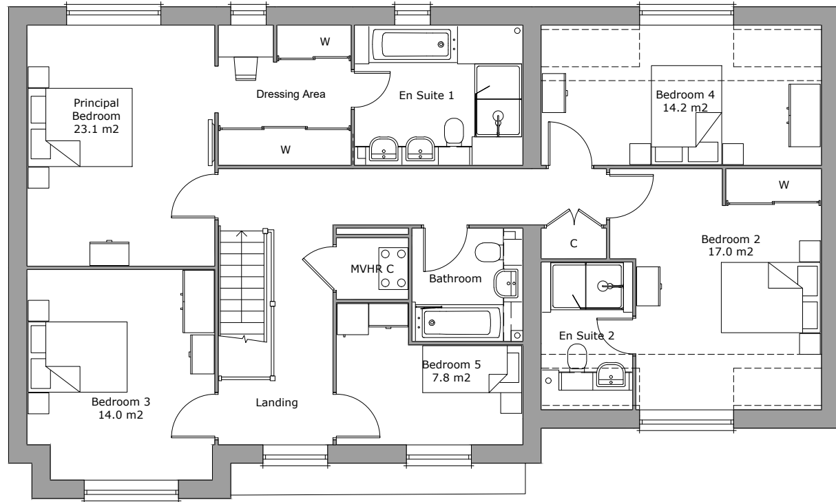
First Floor Plan Area 121.3m²
