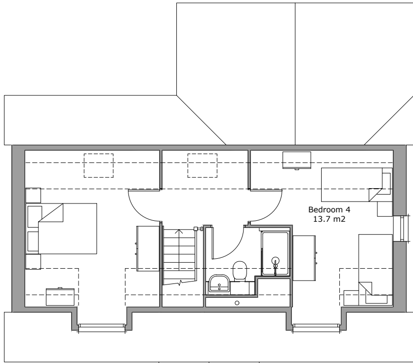
Second Floor Plan Area 42.7m²
