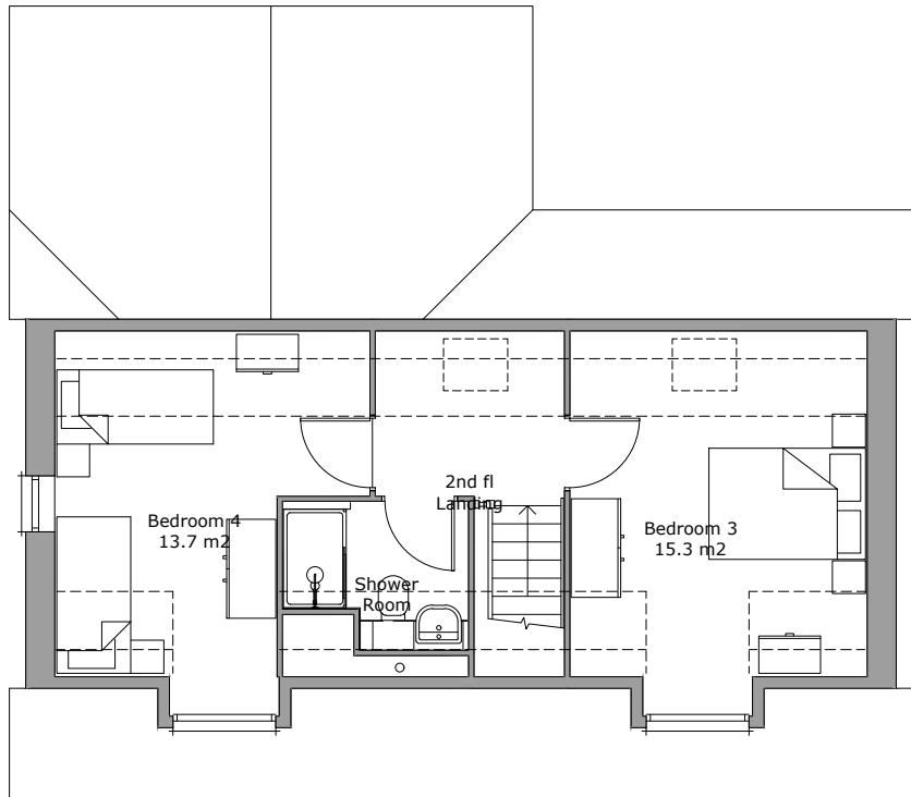
Second Floor Plan Area 41.5m 2
