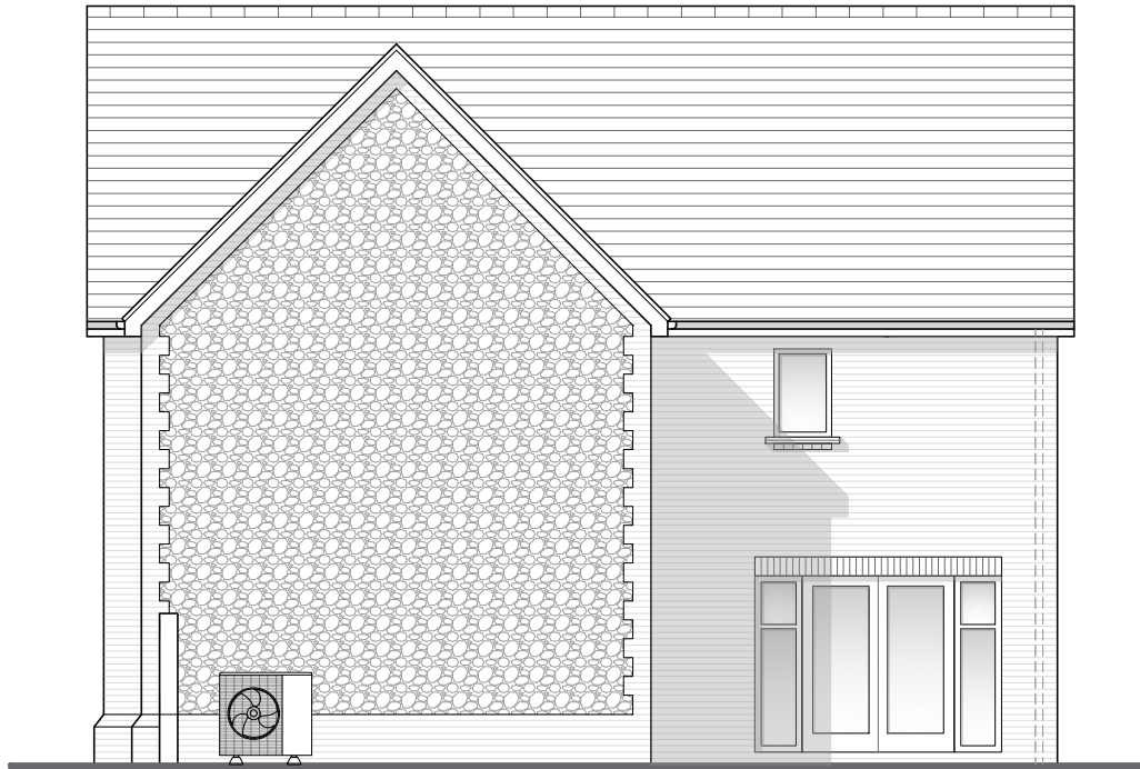
Elevation C
