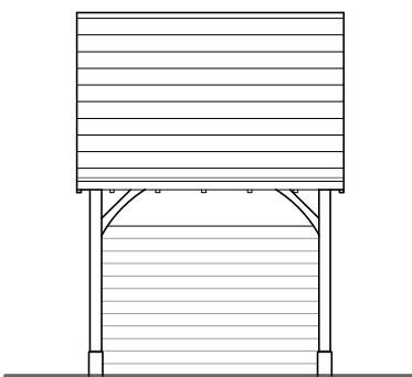
Elevation C
