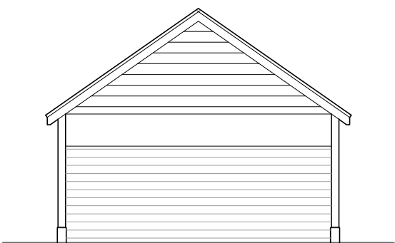
Elevation D
