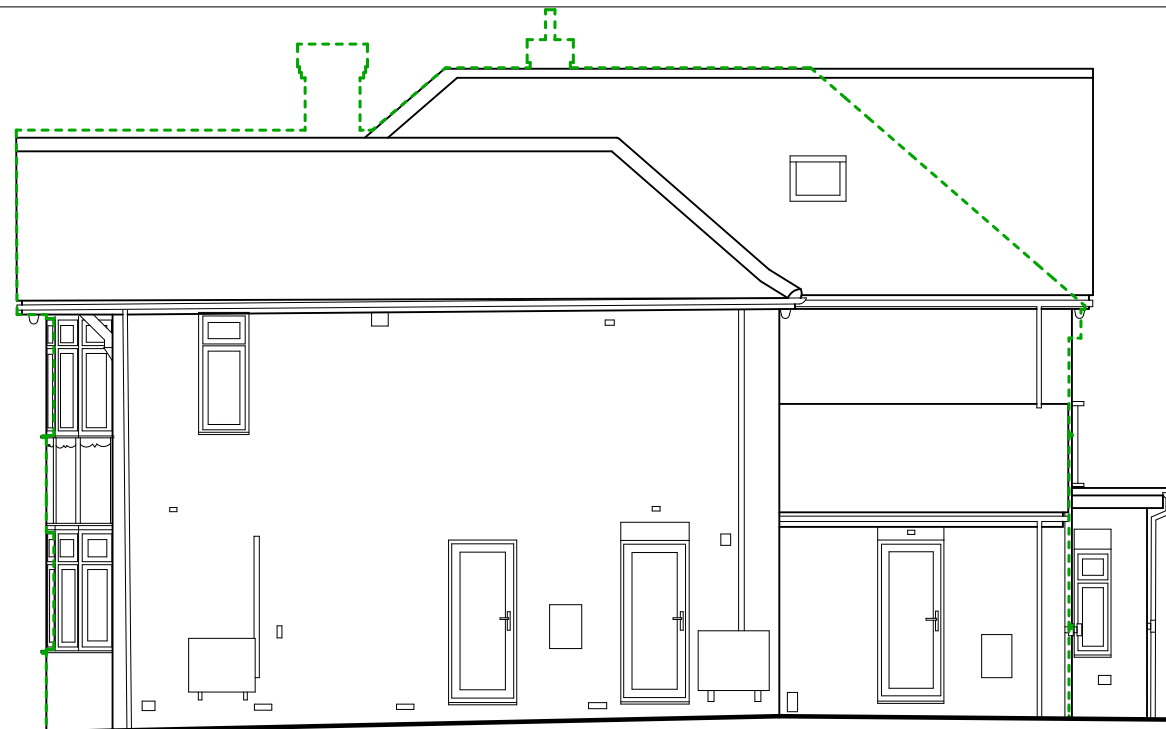
EAST ELEVATION
