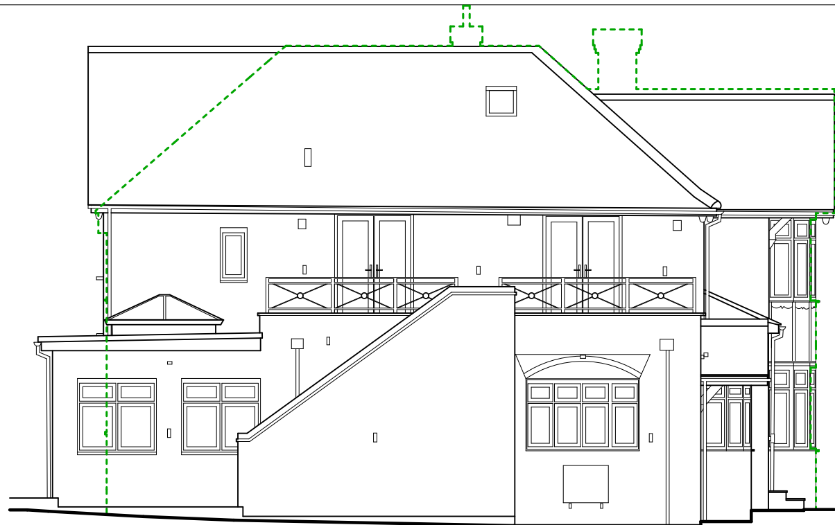
WEST ELEVATION
