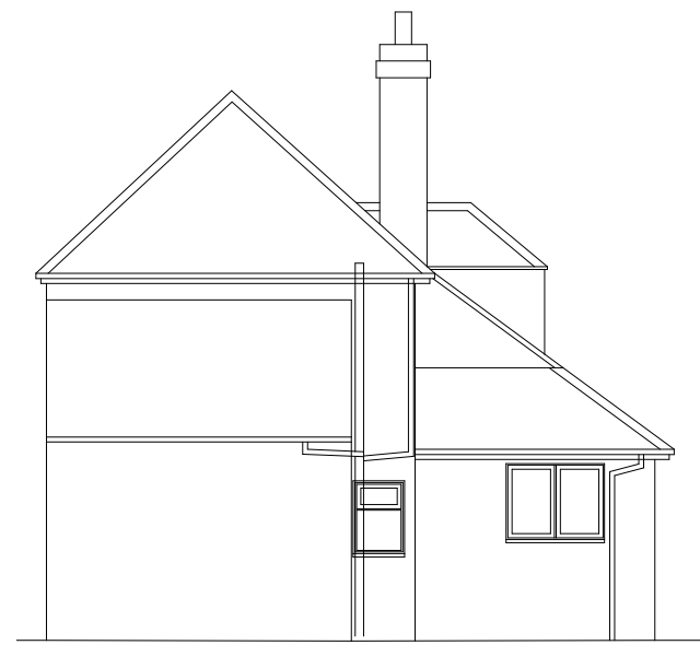
NORTH ELEVATION 1:100
