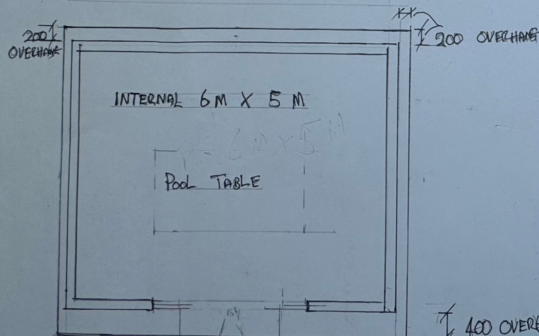
PROPOSED PLAN
