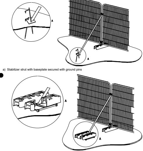
Figure 3 Examples of above-ground stabilizing systems
