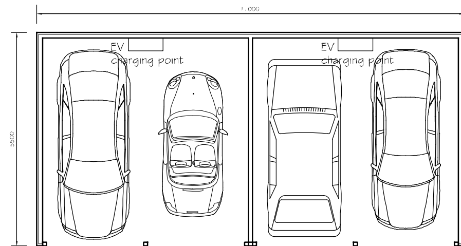
FLOOR PLAN
