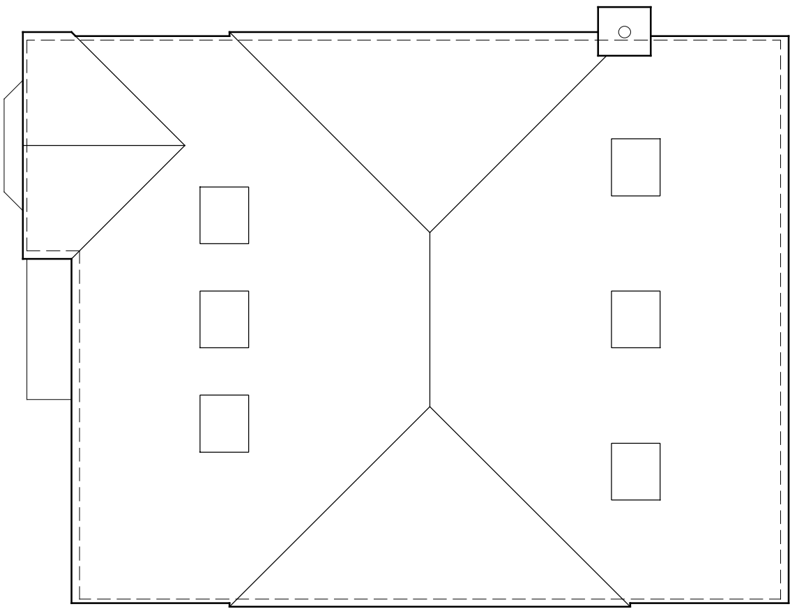
ROOF PLAN
