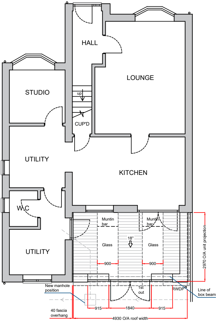
PLAN
