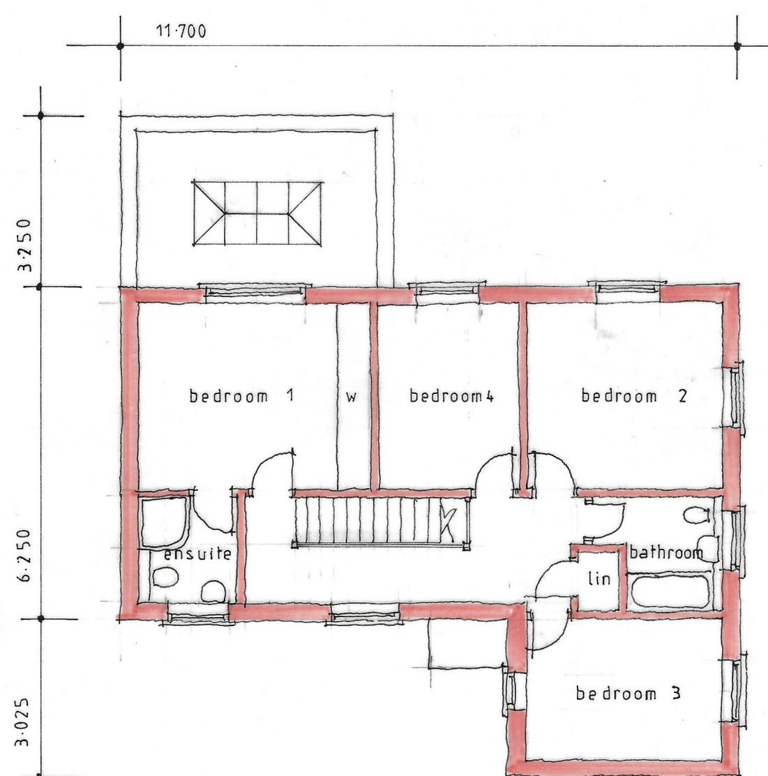
FIRST FLOOR
