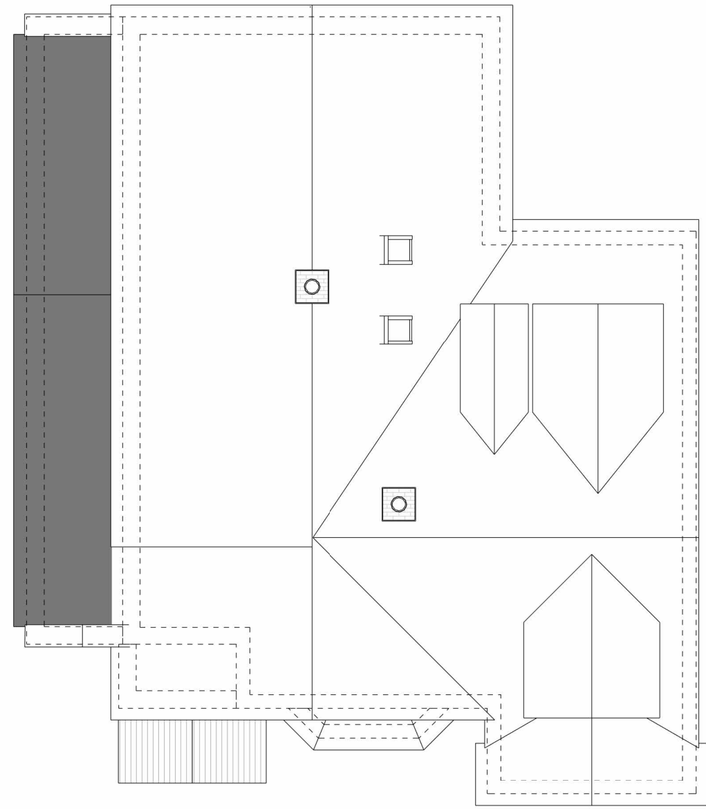
ROOF PLAN
