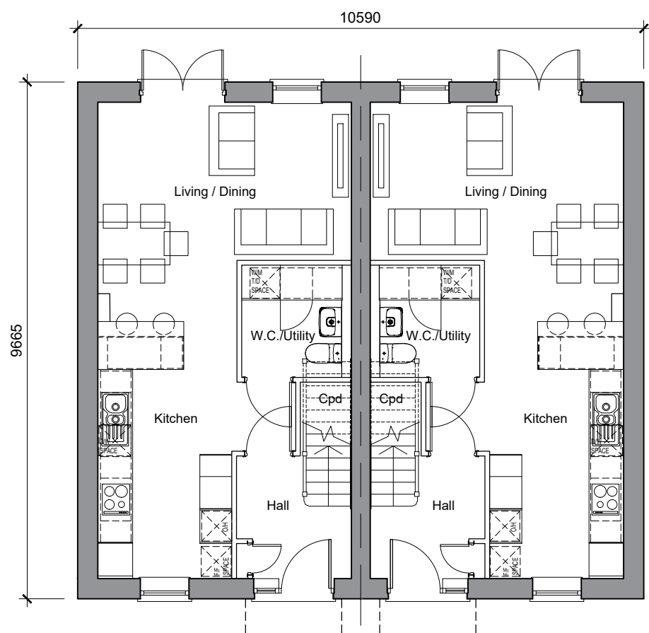
PH3D - 3 Bedroom House NA 113.82sqm Ground Floor Plan Plots 02-03, 46-47, 48-49, 73-74
