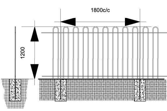
1.2m High Roll Top Railings
