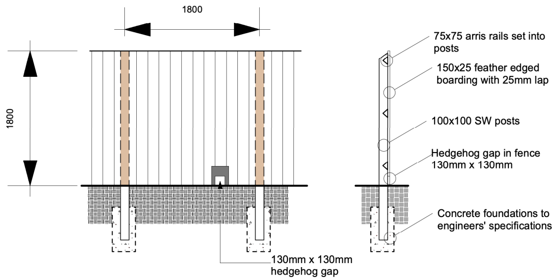
1.8m High Close Board Fence with hedgehog gap
