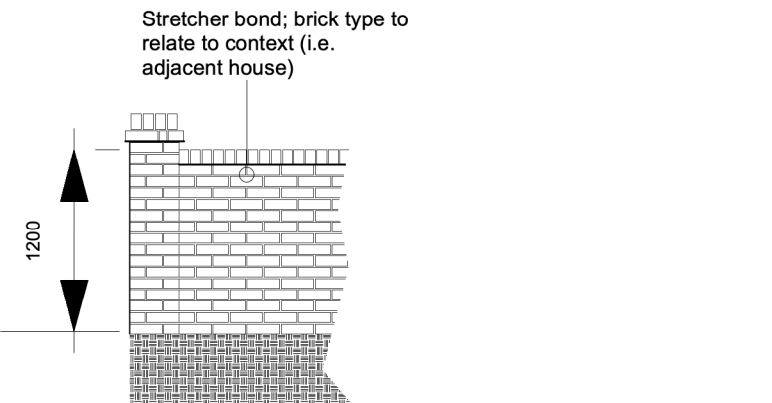
1.2m Low height wall with piers to car park entrances
