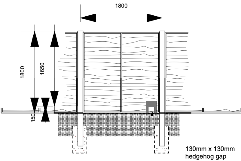
1.8m High larch lap panel fence with hedgehog gap
