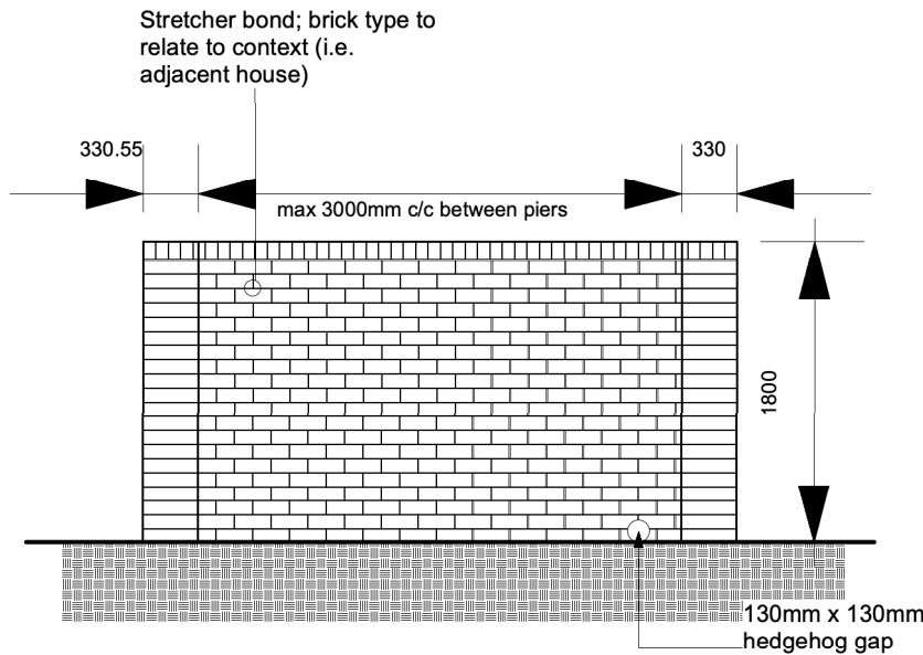
1.8m High brick wall with hedgehog gap
