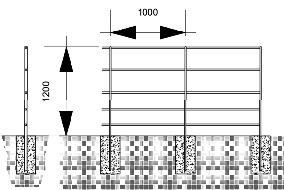
1.2m High Metal Estate Railings
