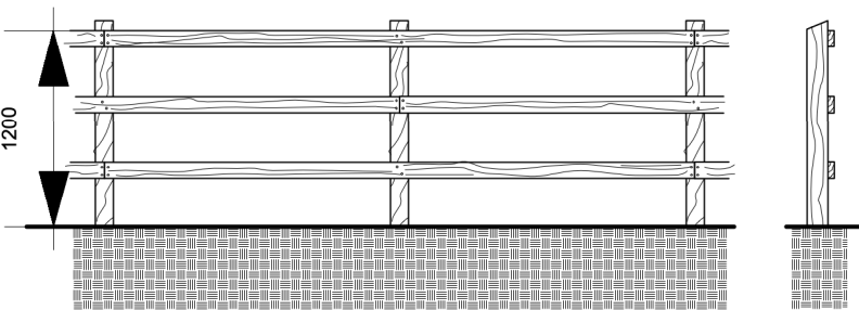
1.2m Timber Post and Rail Fence
