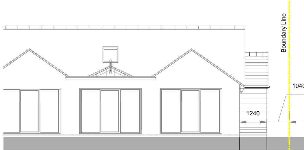
Proposed part west elevation 1:100
