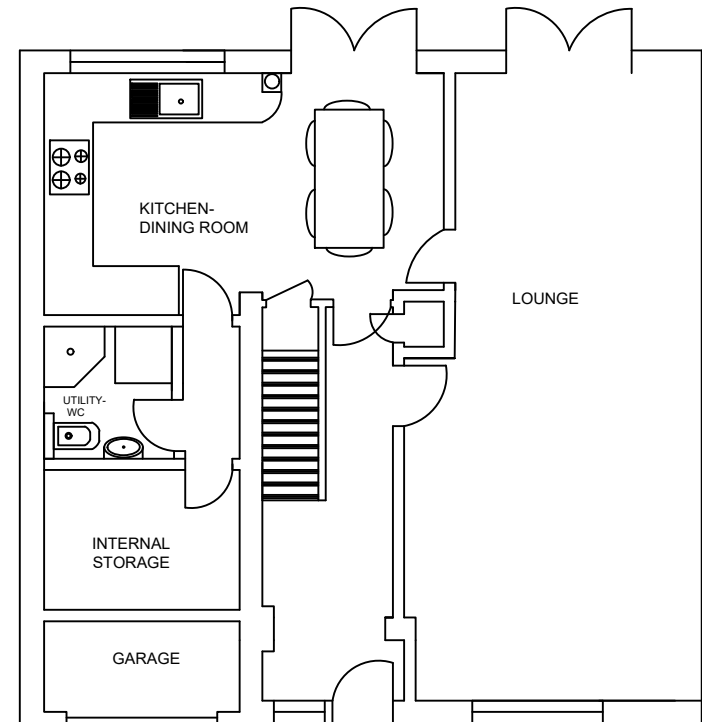
PROPOSED PLAN
