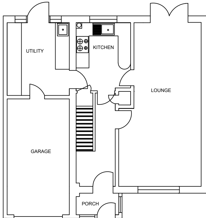
EXISTING PLAN
