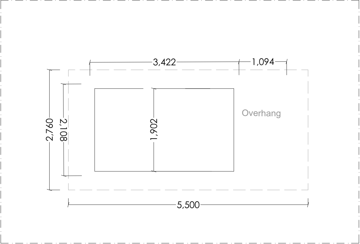
1:50 Ground Floor Shed
