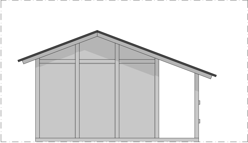
1:50 Proposed Shed Rear Elevation
