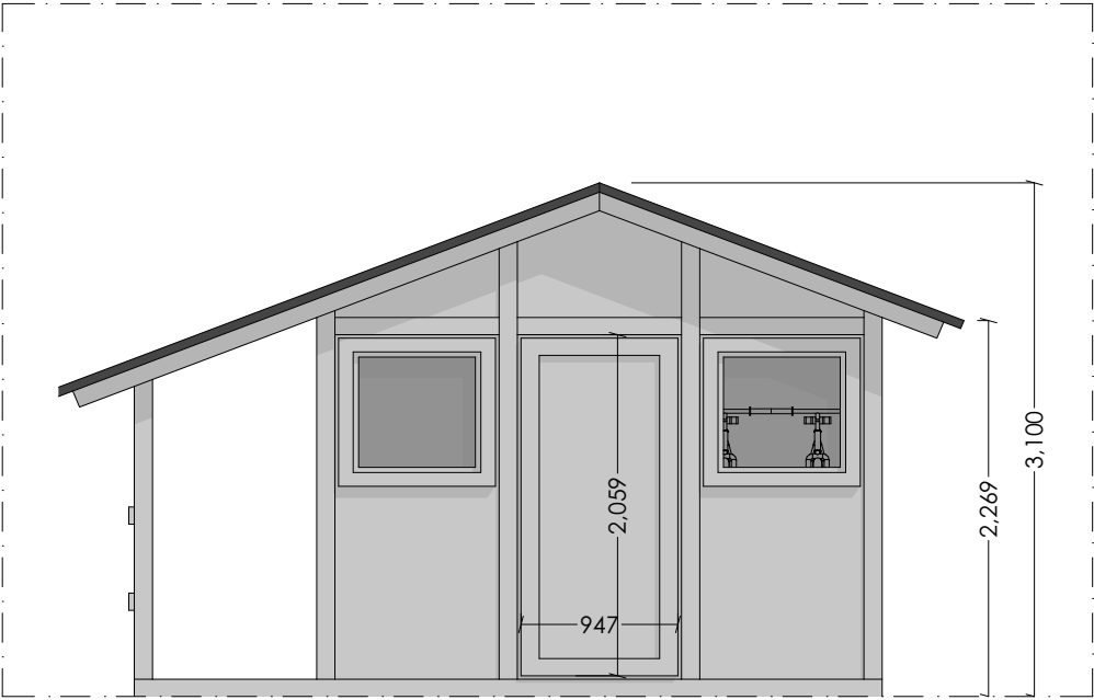
1:50 Proposed Shed Front Elevation
