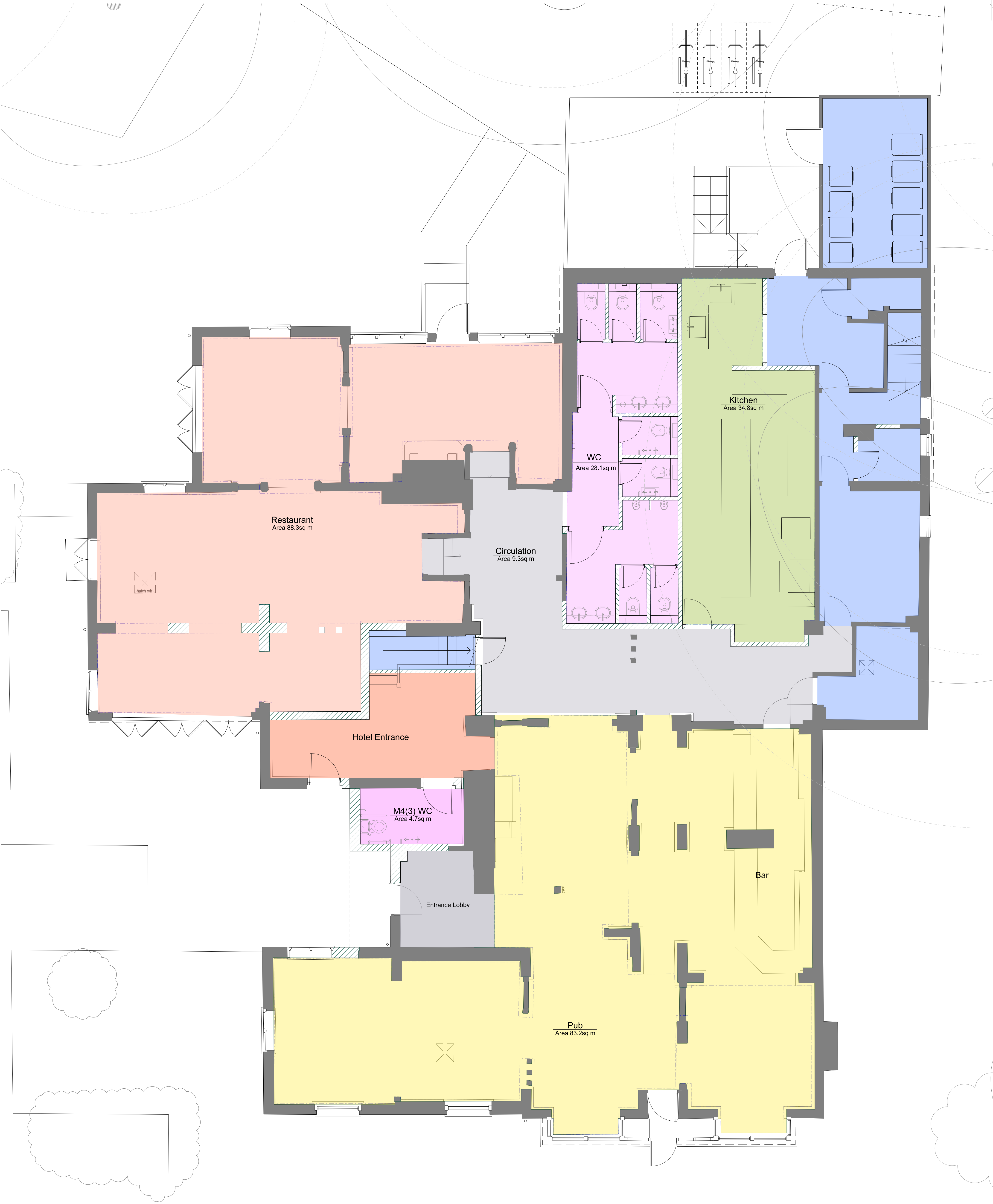
01 Proposed Ground Floor
