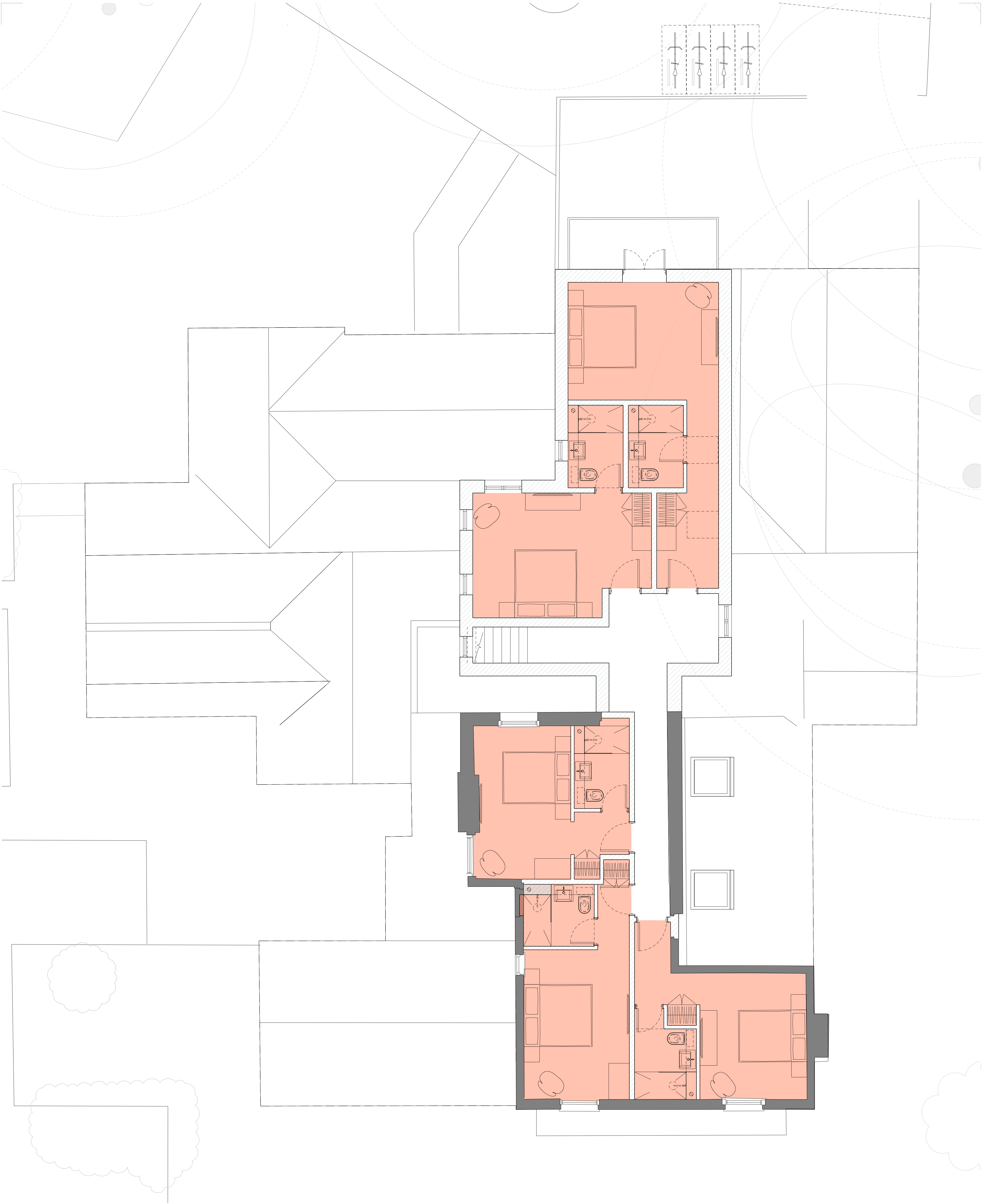
01 Proposed First Floor 03-2003 SCALE 1:50
