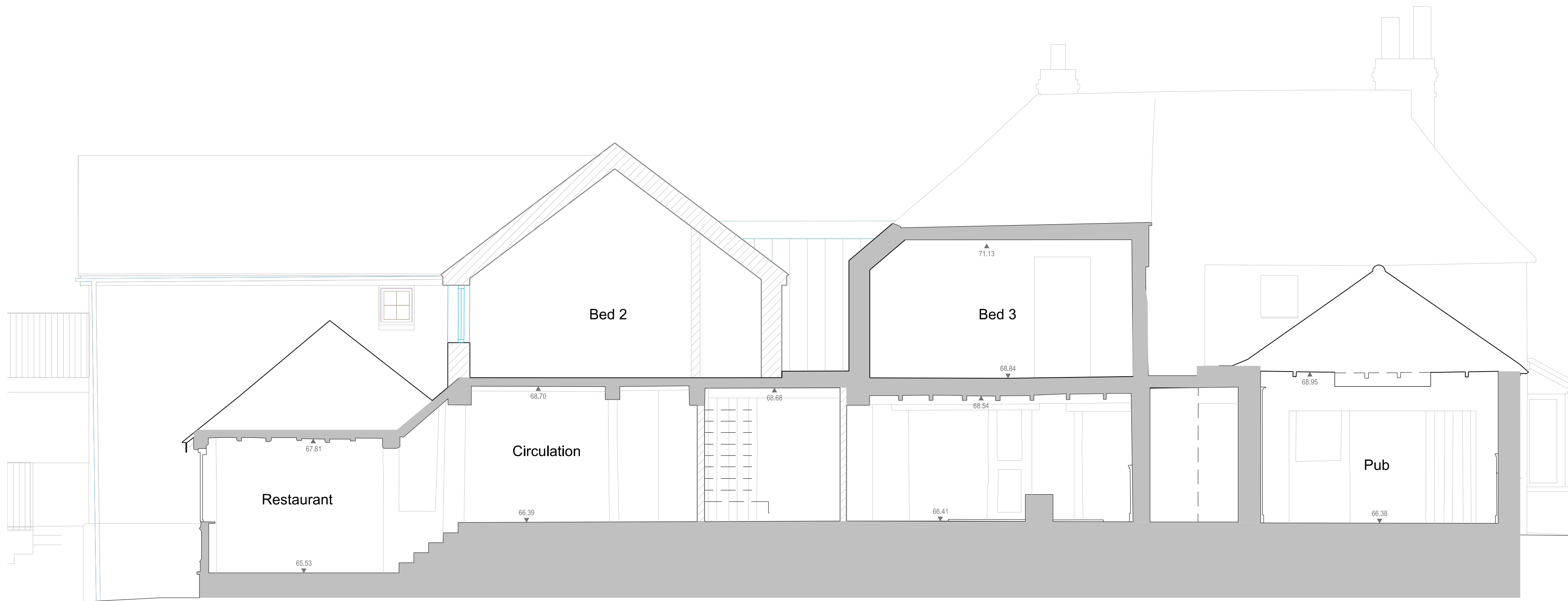
01 Proposed Section C-C 05-2002 SCALE 1:100
