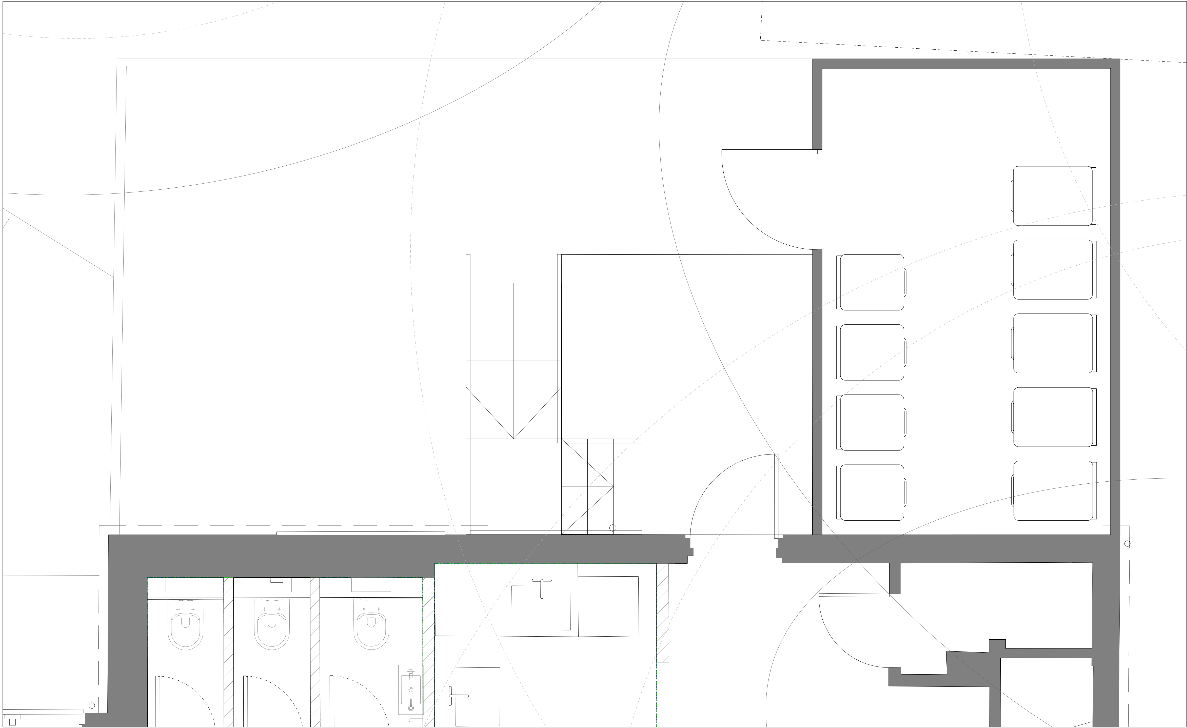
01 Refuse & Recycling Storage Area LWD02-4001 SCALE 1:20
