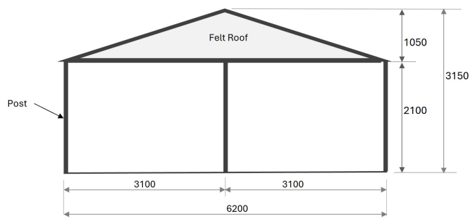
Side Elevation ( Identical from either side )
