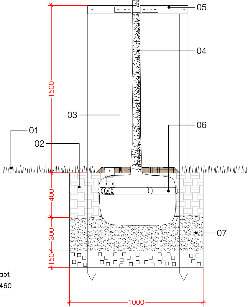
Tree Pit Detail - Soft Landscaping/Staked 1:20 @ A1
