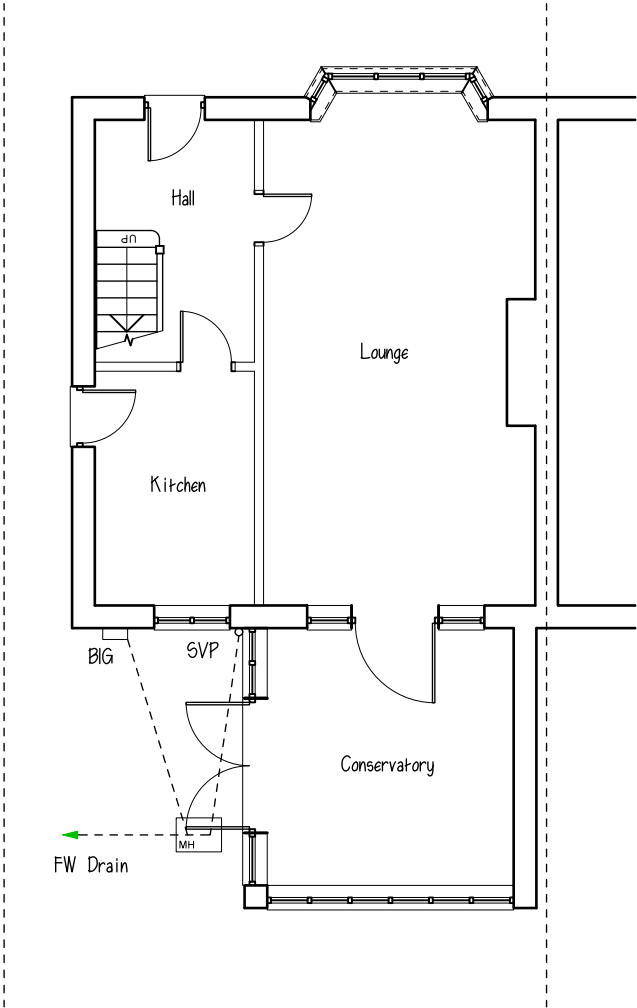
Extg GF Plan
