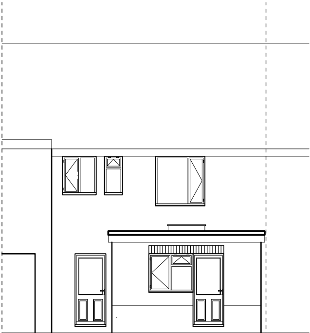
Proposed Rear Elev
