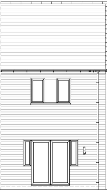
Rear Elevation
