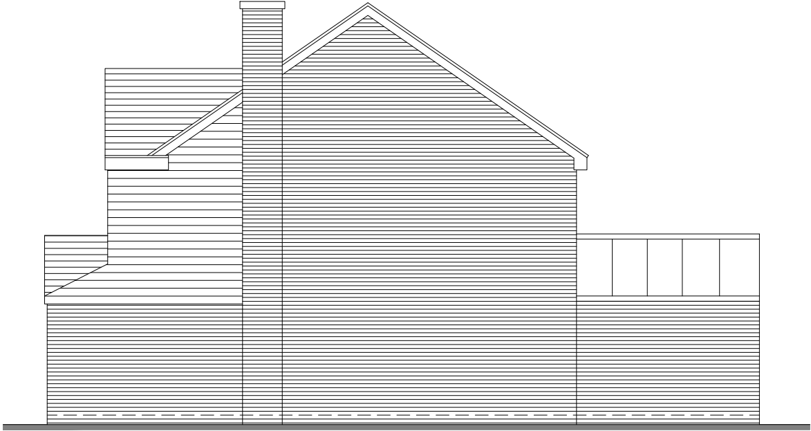
Side Elevation
