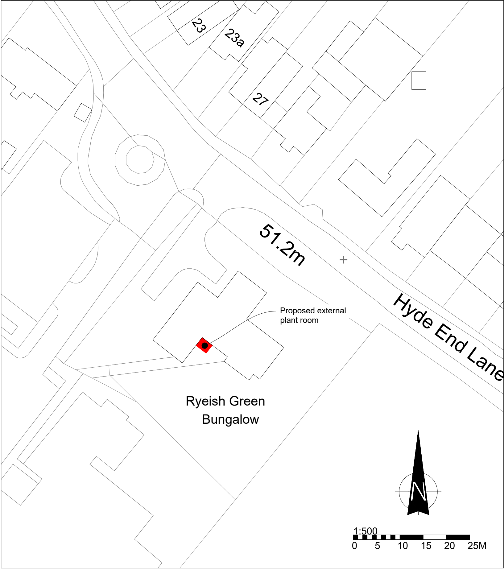
SITE PLAN - 1:500 @ A3
