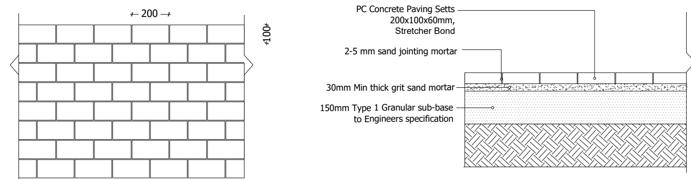
P3 301 PC CONCRETE PAVING SETTS 1:20@A1
