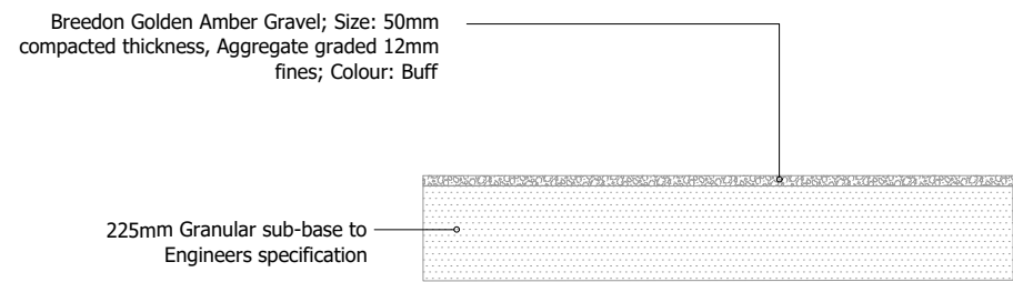
P6 301 SELF BINDING GRAVEL 1:20@A1
