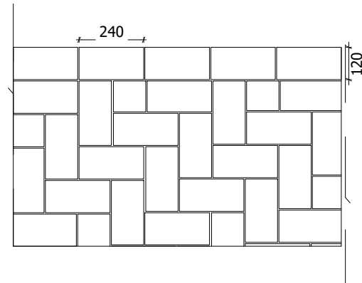
P4 301 PERMEABLE BLOCK PAVING 1:20@A1
