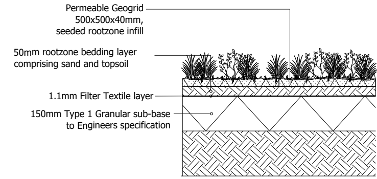
P10 Geogrid with E1 Flowering Lawn
