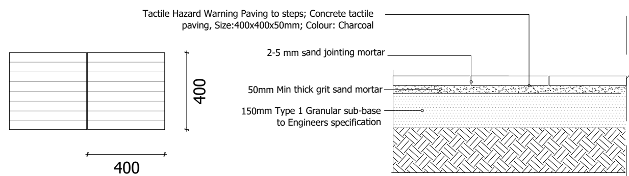
TA1 301 TACTILE PAVING SCALE 1:20@A1
