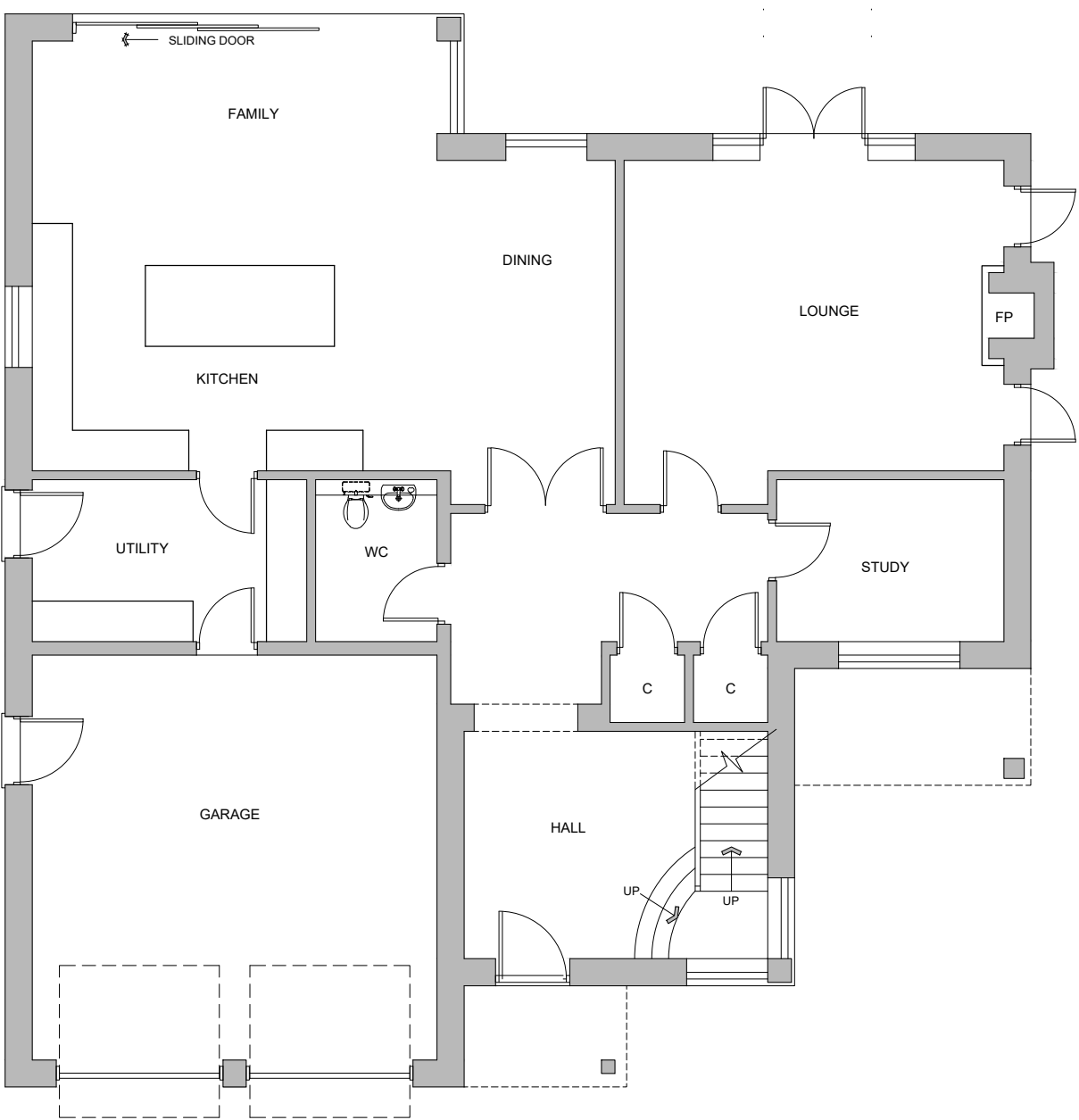
PLOT 1 GROUND FLOOR PLAN
