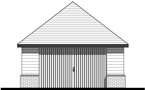
FRONT ELEVATION 1:100 Brooklands, Warren Lane, Finchampstead RG40 4HS
